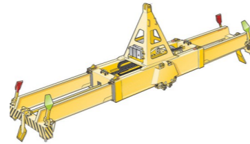
Container spreader
